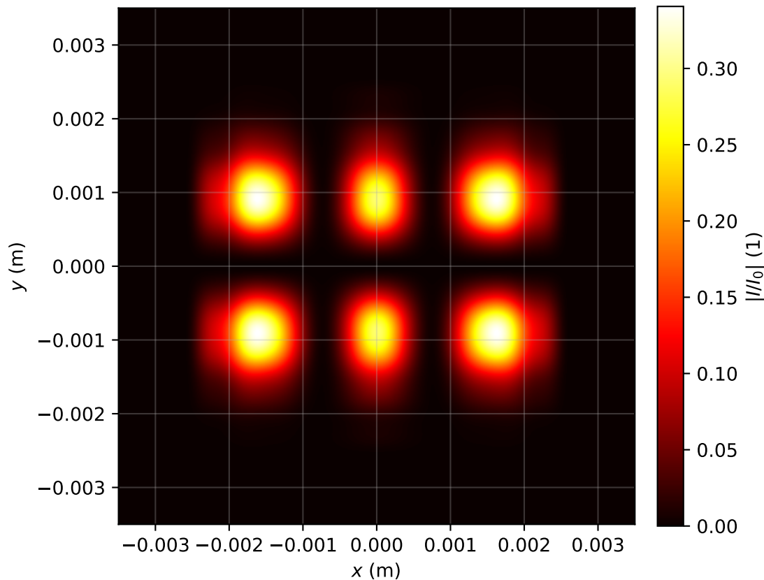
Intensity profile I(x, y, z = 3.503)/I_0 , P_{in}=2.0P_{cr} , artificial time
